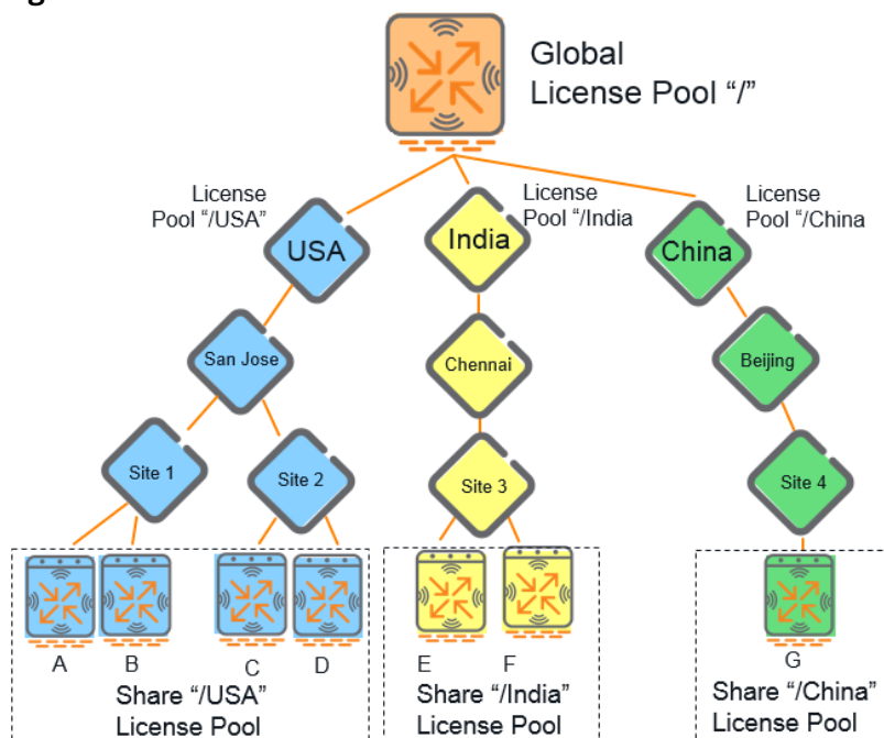
Figure 5 All switches Use a Custom License Pool
